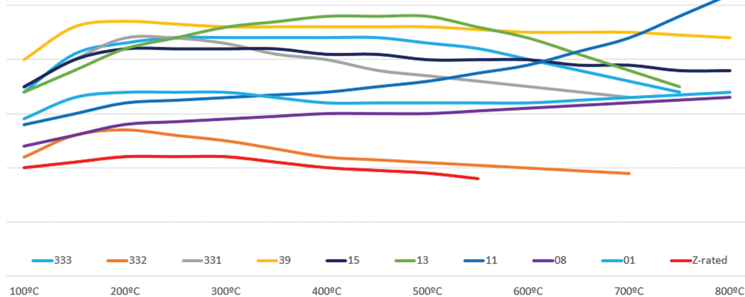
Friction vs temperature
